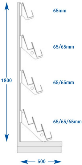
8 Tiered Super
